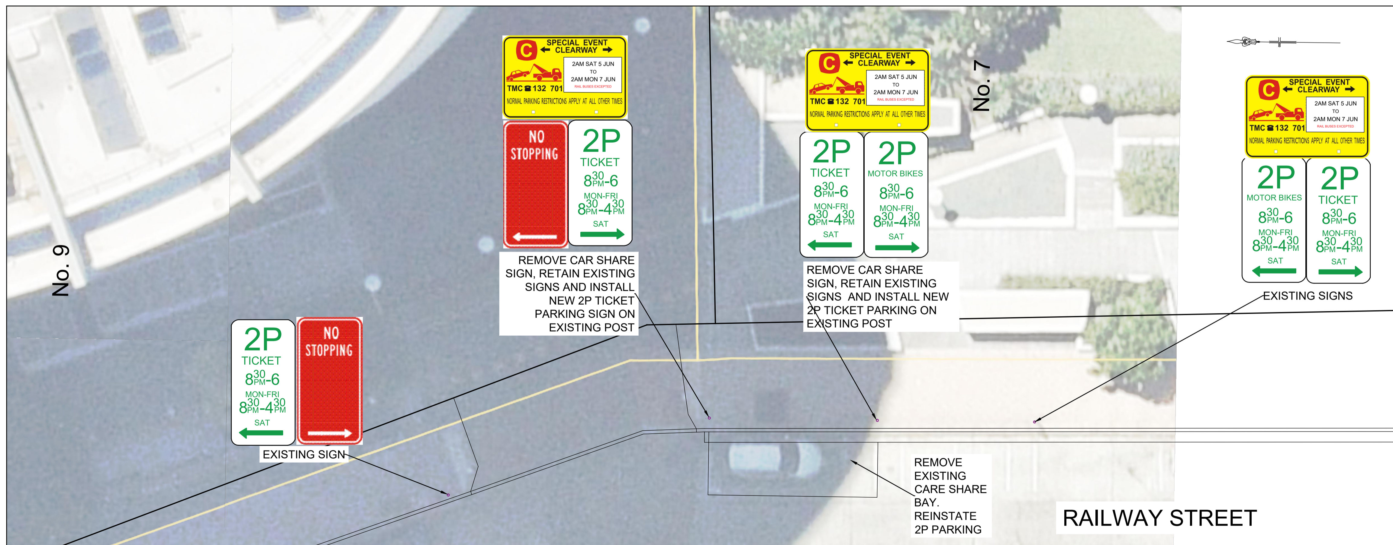
PLAN SCALE 1:100
