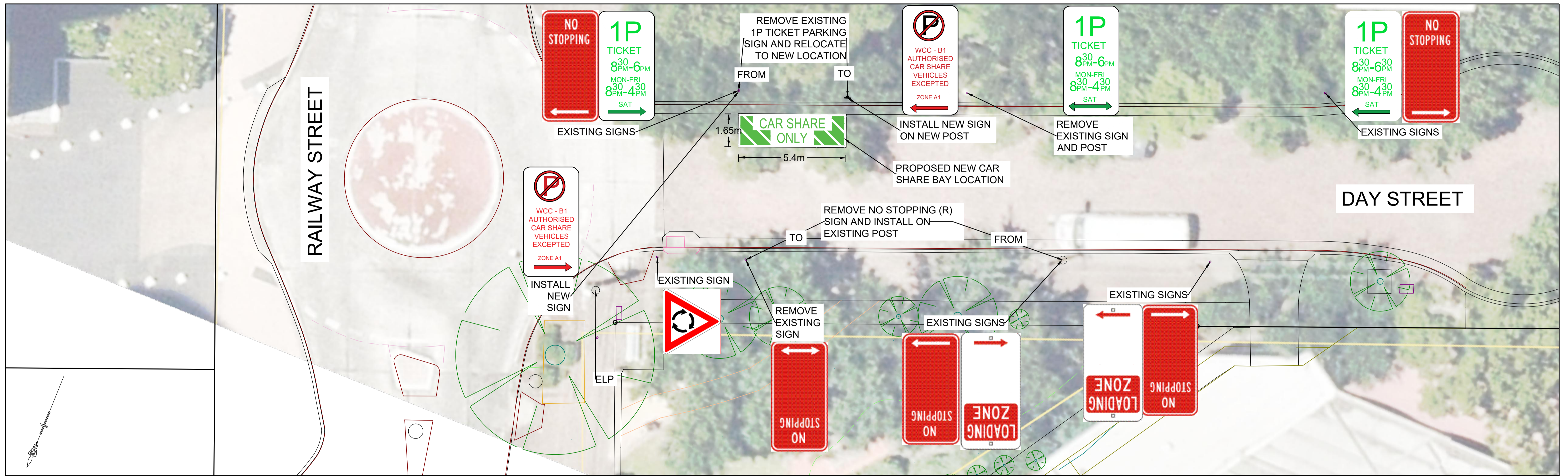
PLAN SCALE 1:100
