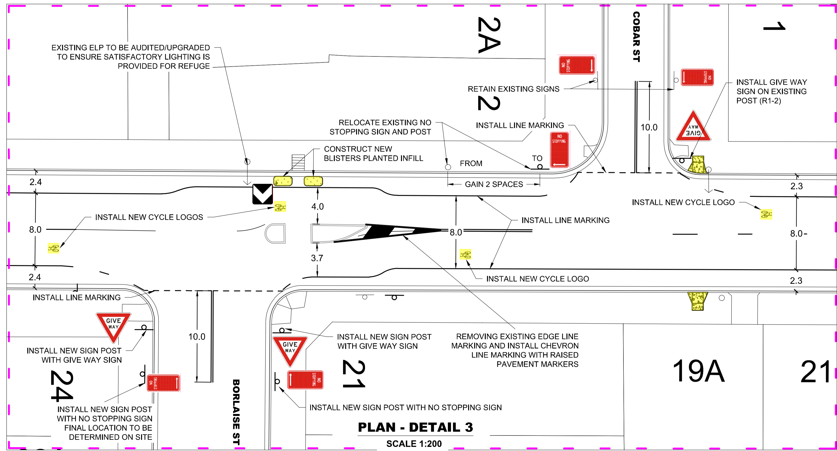
PLAN - SECTION 2 SCALE 1:400
