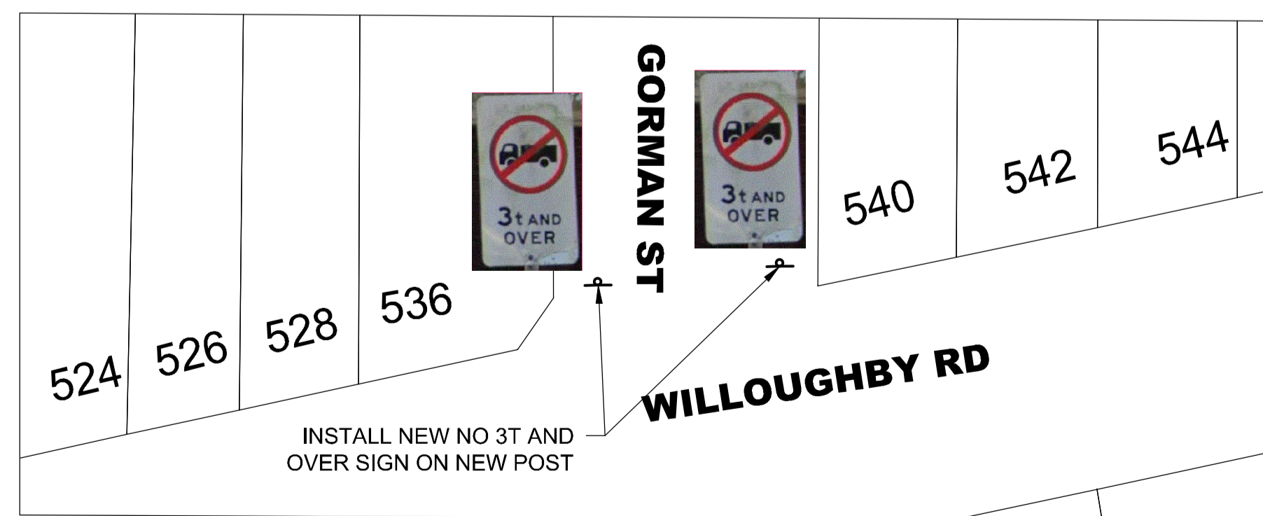
PLAN - NO 3T AND OVER SIGNAGE INSTALLATION GORMAN ST AND WILLOUGHBY RD SCALE 1:400
